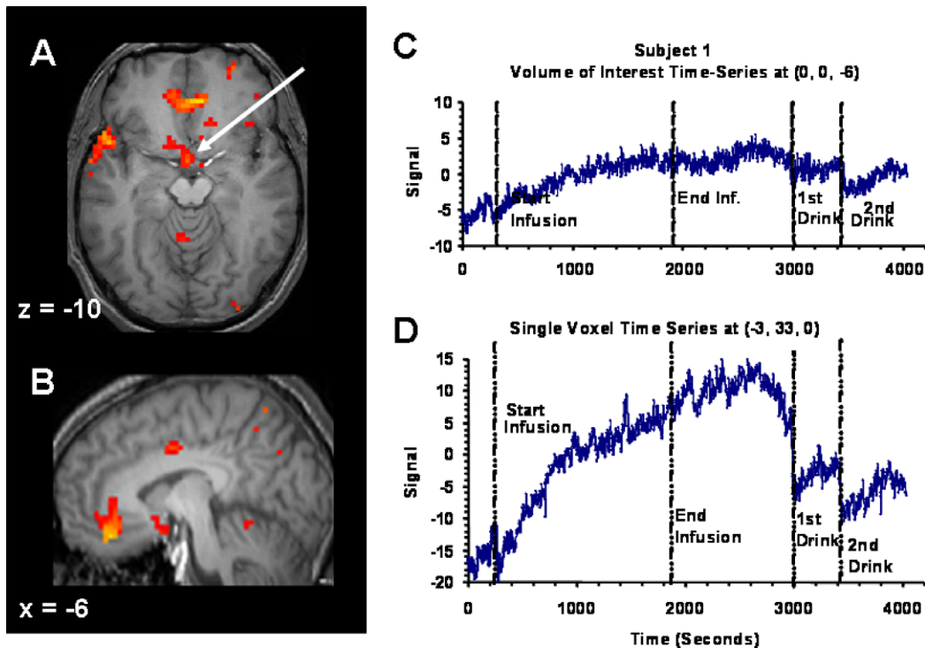
Fig. 3. Functional magnetic resonance images (fMRI) using blood oxygen level-dependent (BOLD) contrast were acquired over 60 min prior to, during and after systemic infusion of 0.51 M NaCl in a healthy male. Activations were generated by contrasting the period of maximum increase of thirst with scans acquired during the pre-infusion baseline state. (A) Maximum thirst activations were present in a region of the hypothalamus incorporating the lamina terminalis (indicated by arrow). (B) The anterior cingulate cortex (BA 32) was also activated during maximum thirst. (C) The BOLD signal from a voxel in the hypothalamus increased during the infusion and remained elevated after drinking. (D) The time course of the BOLD signal from a voxel in the anterior cingulate cortex indicates a rise in response to the hypertonic infusion, that was reversed after drinking. Co-ordinates in (A) and (B) are distances in mm from the anterior commissure according to the Talairach and Tournoux stereotactic reference system (Talairach & Tournoux, 1988). Figure adapted from Egan et al. (2003).
