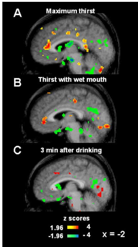
Fig. 1. Positron Emission Tomography (PET) measures of regional cerebral blood flow (rCBF) were made before (baseline), during and after systemic infusion of 0.51 M NaCl in 10 healthy men. (A) Contrasting the period of maximum thirst with baseline scans produced activation in Brodmann Area (BA) 32 of the anterior cingulate cortex and midcingulate and posterior cingulate region. (B) Activation was still present in BA 32 when scans acquired after rinsing the mouth with water were contrasted with baseline. (C) The contrast between the immediate post drink period and baseline did show disappearance of the activation in BA 32 contemporaneous with the loss of thirst. Activations are rendered on an average of the 10 subjects' anatomical images after normalization to the Talairach and Tournoux stereotactic reference system (Talairach & Tournoux, 1988). The sagittal section is 2 mm to the left of the anterior commissure. Figure adapted from Denton et al. (1999a), Denton et al. (1999b).
