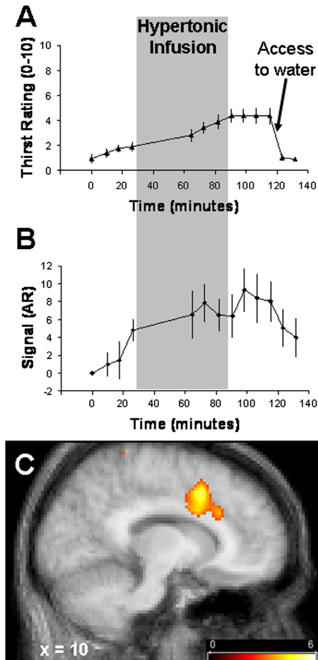
Fig. 2. (A) A systemic infusion of 0.51 M NaCl in 10 healthy mean was associated with increased ratings of thirst that rapidly decreased after drinking. (B) PET measures of rCBF in voxels activated during maximum thirst show a pronounced decrease in signal intensity after drinking. (C) The voxels activated by maximum thirst were located in the mid cingulate cortex, approximately 10 mm from the midline into the right hemisphere. Figure adapted from Farrell et al. (2006).
