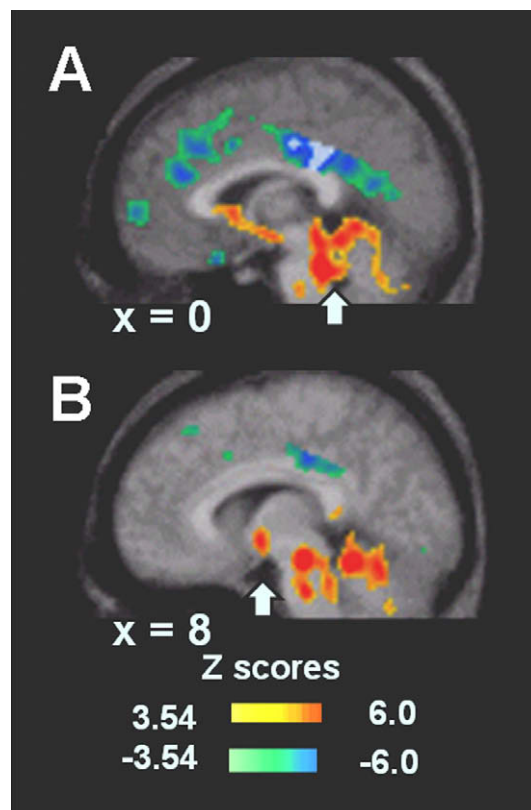
Fig. 5. Air-hunger activations were identified by contrasting PET measures of rCBF from scans acquired during inhalation of 8% CO 2 with scans acquired during inhalation of a N 2 /O 2 mixture. (A) Air-hunger activations included an extensive region of the midbrain and brainstem (indicated by arrow) that incorporated the midbrain tegmentum, periaqueductal grey and pons. (B) Air hunger was also notable for activation in the hypothalamus (indicated by arrow). The x values represent the lateral position in mm of the sagittal slice with respect to the anterior commissure, according to the Talairach and Tournoux stereotactic reference system (Talairach & Tournoux, 1988). Figure adapted from Brannan et al. (2001).
