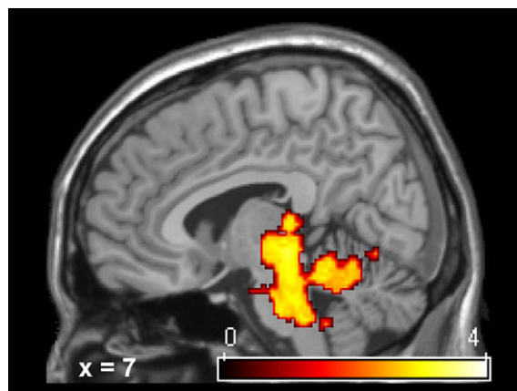
Fig. 4. Measures of rCBF were collected with a pulsed arterial spin labelling (PASL) magnetic resonance imaging sequence in 15 healthy subjects, immediately after eating to satiation following an 18 h fast and then 90 min after eating. Satiation activations were identified by contrasting images acquired immediately after eating with those acquired 90 min after eating, which acted as control. An extensive region of midbrain, brainstem and cerebellum was activated during the satiation period. Sagittal slice is 7 mm lateral to the anterior commissure in the right hemisphere. The activation is rendered on the Montreal Neurosciences Institute template brain. Image has been generated from unpublished data.
