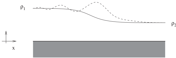
Figure 1. Schematic of geometry of initial-value problem. The solid curve shows the function h(x) . The dashed curve represents a possible surface profile, and the grey shaded area represents the river bed.
