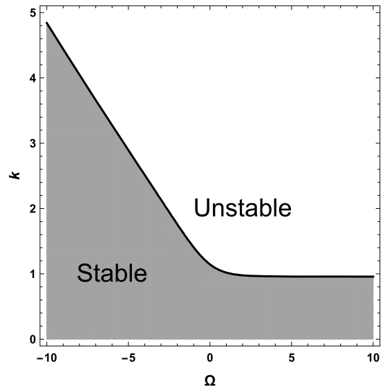
Fig. 9. Stability diagram in the (\Omega, k) -plane for small-amplitude, periodic, traveling-wave solutions to the vor-Whitham equation.
