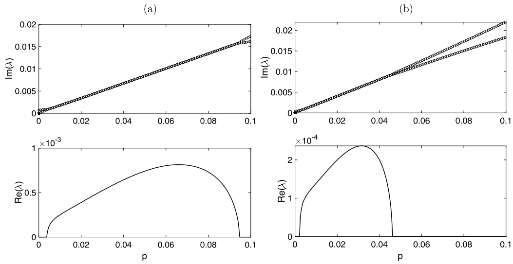
Fig. 5. Radian frequency (top) and rate of growth (bottom) of the normal mode perturbation against its wavenumber for ak = 0.20 and (a) \Omega = -0.1 (b) \Omega = 0.1 .
