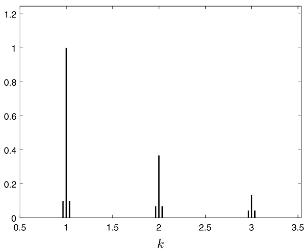
Fig. 7. Amplitude spectrum of the unperturbed wave of wave steepness ak = 0.20 perturbed by its most unstable normal mode for \Omega = 0.1 . The amplitudes of the Fourier components have been normalized by the amplitude of the fundamental mode k = 1 of the unperturbed wave.
