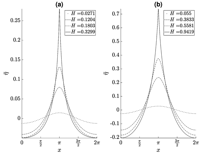
Fig. 1. Plots of periodic traveling-wave solutions to the vor-Whitham equation with L = 2\pi , wave height, H (see captions), and (a) \Omega = -1.0 , (b) \Omega = 1.0 . Note that the vertical scales in the two plots are different.
