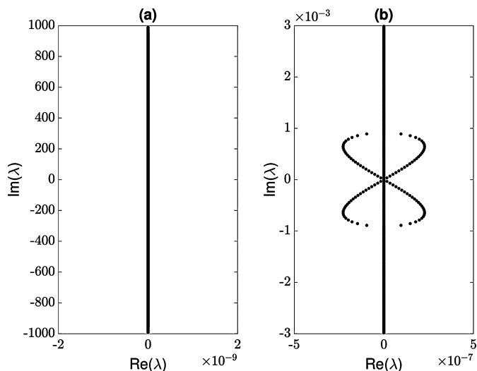
Fig. 10. Stability spectra for (a) a small-amplitude solution to the vor-Whitham equation with (\Omega, k) = (5, 0.9) and (b) a small-amplitude solution to the vor-Whitham equation with (\Omega, k) = (5, 1) . Note that the axes in the two plots are scaled differently. The spectrum in (a) lies purely on the imaginary axis and therefore the corresponding solution is spectrally stable. The spectrum in (b) has values with positive real parts and therefore the corresponding solution is unstable.
