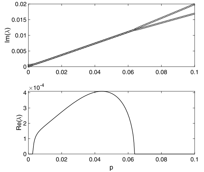
Fig. 4. Radian frequency (top) and rate of growth (bottom) of the normal mode perturbation against its wavenumber for \Omega = 0 and ak = 0.20 .
