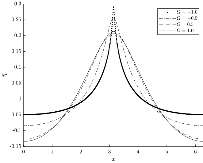
Fig. 2. Plots of periodic traveling-wave solutions to the vor-Whitham equation with wave height, H = 0.34 , L = 2\pi , and four different values of \Omega .
