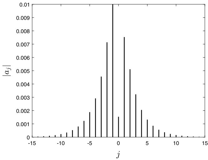
Fig. 6. Magnitude of the coefficient a_j of the most unstable normal mode corresponding to \Omega = 0.1 and ak = 0.20 .
