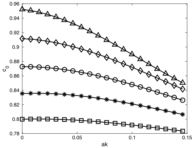
Fig. 3. Phase velocity of the traveling-wave solutions as a function of the wave steepness for several values of the vorticity. \Omega = 0 ( \circ ), -0.1 ( * ), 0.1 ( \diamond ), -0.2 ( \square ), 0.2 ( \triangle ).
