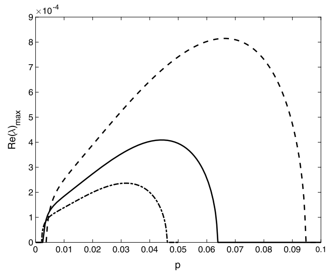
Fig. 8. Maximum growth rate against the wavenumber for \Omega = 0 (solid line), \Omega = -0.1 (dashed line), \Omega = 0.1 (dot-dashed line) and ak = 0.20 .
