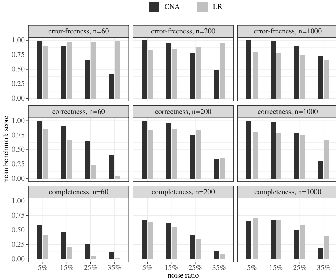
Figure 1: Bar-plots displaying mean scores of Coincidence Analysis (CNA; in black) and Logic Regression (LR; in grey) in error-freeness (i.e., ratio of trials without false positive), correctness (i.e., ratio of trials in which a correct model is recovered), and completeness (i.e., ratio of the ground truth complexity recovered), averaged over 1000 trials in each test type, broken down by noise levels (on x -axis) and sample sizes (from left to right). These means have standard errors between 0.0004 and 0.015.
