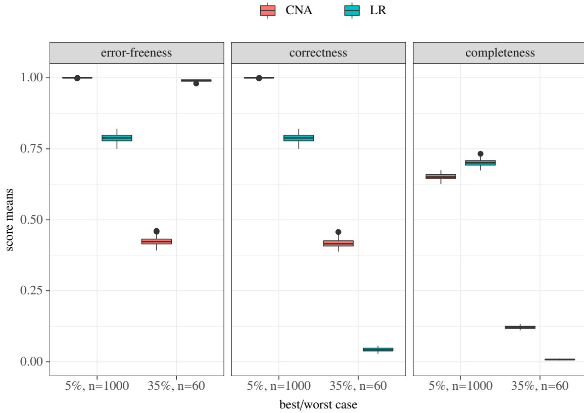
Figure S2: Box-and-whisker plots showing the distribution of mean benchmark scores obtained from 60 replications of the trials on data of types \delta_{1000}^{5\%} and \delta_{60}^{35\%} (i.e., the best and worst case trials) simulated from 1000 different ground truths each. Boxes represent the IQR (i.e., inter-quartile range between the 25 th and 75 th percentile). Whiskers extend to 1.5 \times IQR. Dots represent outliers.
