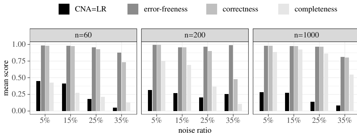
Figure 2: Black bars represent the ratios of trials in which Coincidence Analysis (CNA) and Logic Regression (LR) produce an identical model. Increasingly lighter shades of grey represent the error-freeness, correctness, and completeness scores reached by the subpopulation of identical models.
