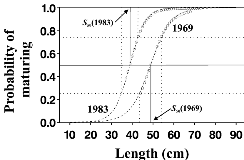
Fig. 3. Application of the estimation method for Georges Bank cod stock. Probability of maturing at age 3 computed as a function of size for cohorts 1969 and 1983. \circ , raw estimations of the probabilities of maturing computed in the observed size range; —, fitted logistic regression curves. Thin solid lines (dotted) indicate how the reaction norm midpoints (quartiles) can be graphically determined.
