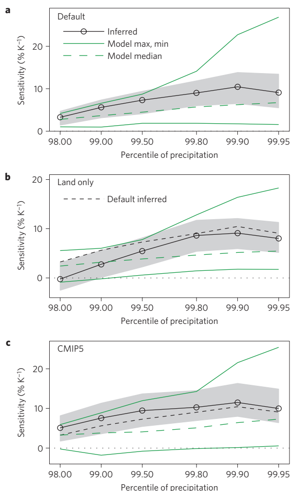
Figure 3 | Inferred and simulated climate-change sensitivities ( \% \text{K}^{-1} ) for high percentiles of precipitation. Black lines with circles show inferred sensitivities, shading shows the associated 90% confidence intervals, solid green lines show multimodel maxima and minima, and dashed green lines show multimodel medians. a , CMIP3 models and the whole tropics. b as in a but for climate change over land only and normalized by temperature changes over the whole tropics. c as in a but for CMIP5 models. Black dashed lines in b,c reproduce the inferred sensitivities shown in a .
