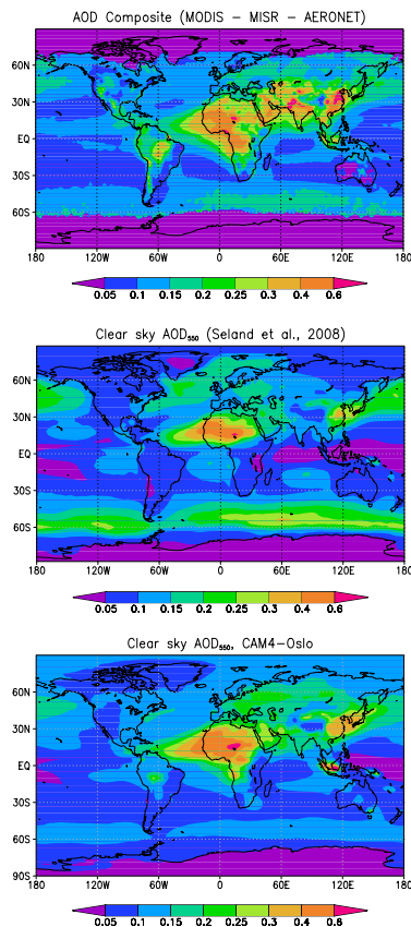
Fig. 7. Annually averaged clear sky aerosol optical depth (AOD) at 550 nm from ground and satellite based retrievals in the upper panel (S. Kinne, personal communication, 2007), as calculated in Seland et al. (2008) in the middle panel, and calculated with CAM4-Oslo ( Ctrl ) in the lower panel.
