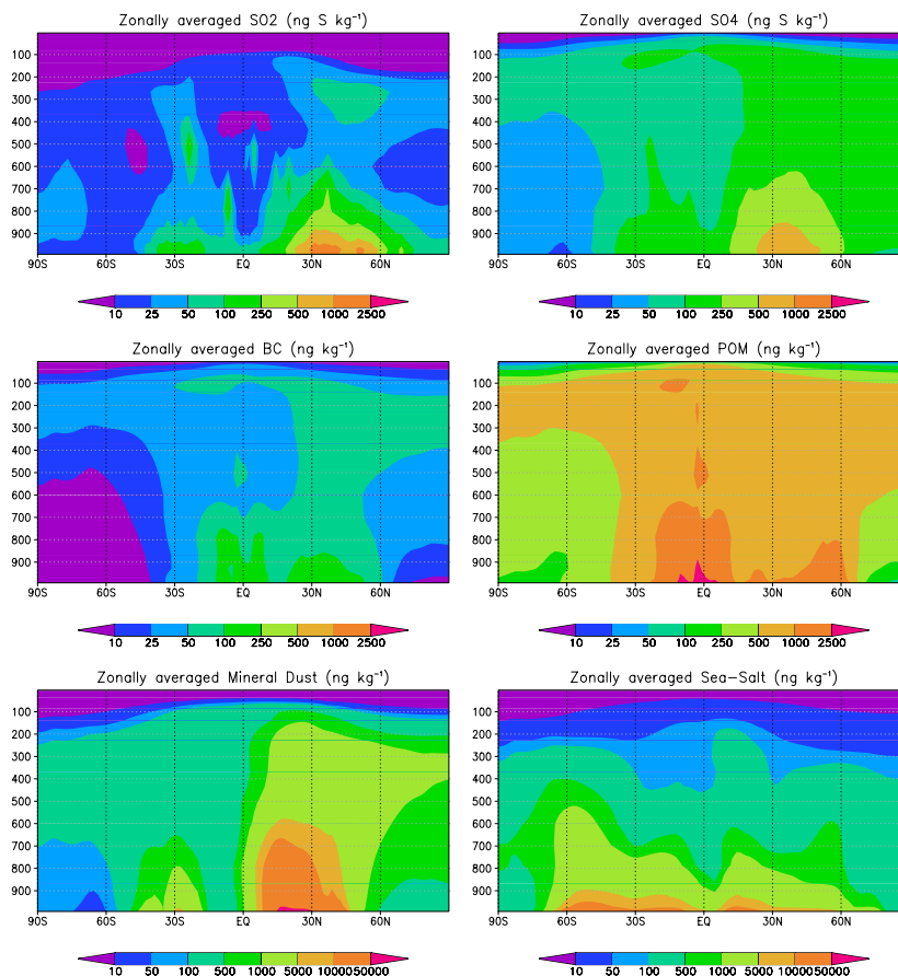
Fig. 3. Annually and zonally averaged mass mixing ratios of SO 2 and aerosol constituents in the Ctrl simulation.
