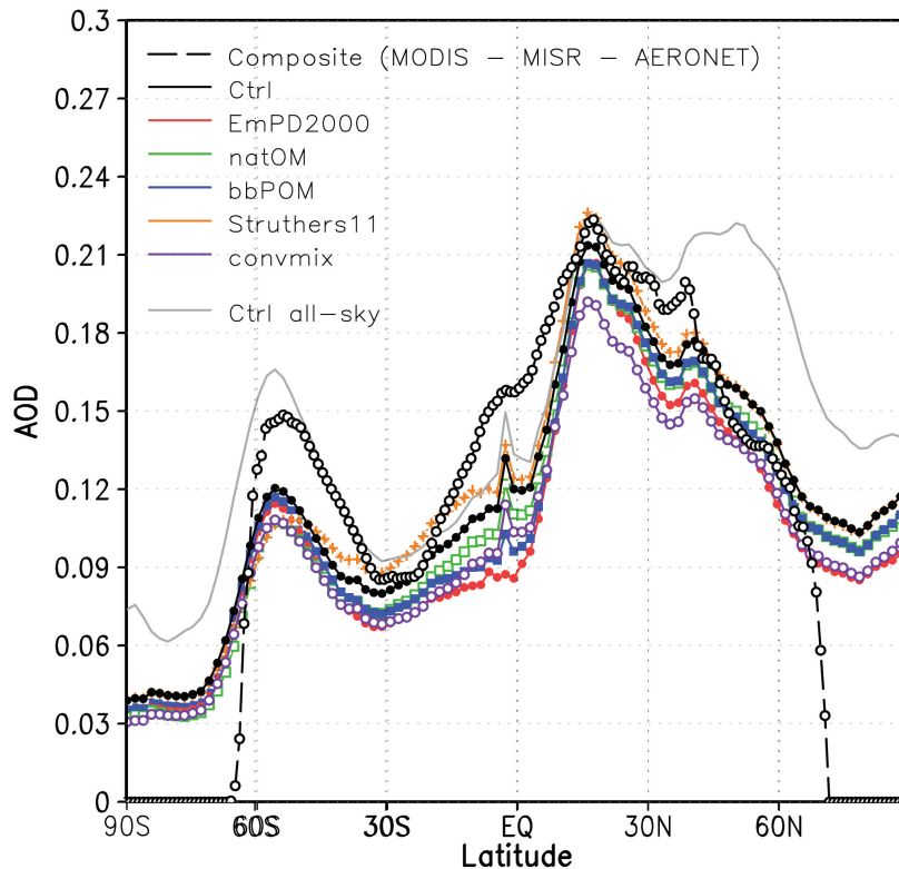
Fig. 6. Zonally and annually averaged clear-sky aerosol optical depth (AOD) at 550 nm from ground and satellite based retrievals (S. Kinne, personal communication, 2007), and calculated with CAM4-Oslo for year 7 of the Ctrl experiment and a selection of sensitivity tests. For comparison with the clear-sky AOD, also all-sky AOD at 550 nm is shown for the Ctrl simulation (gray solid line).
