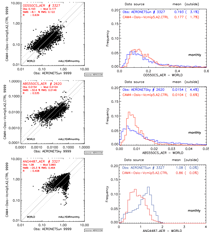
Fig. 9. Model-calculated vs. retrieved aerosol optics data from AERONET, shown as scatter-plots (left) and frequency histograms (right). Upper row: modeled clear-sky AOD at wavelength 550 nm vs. AERONET. Middle row: modeled clear-sky ABS (absorption AOD) at wavelength 550 nm vs. AERONET ABS. Lower row: ANG (Ångström parameter) calculated from all-sky AOD at 440 and 870 nm. The AERONET retrievals are from the period 2000–2009, and are made available through the AeroCom project.
