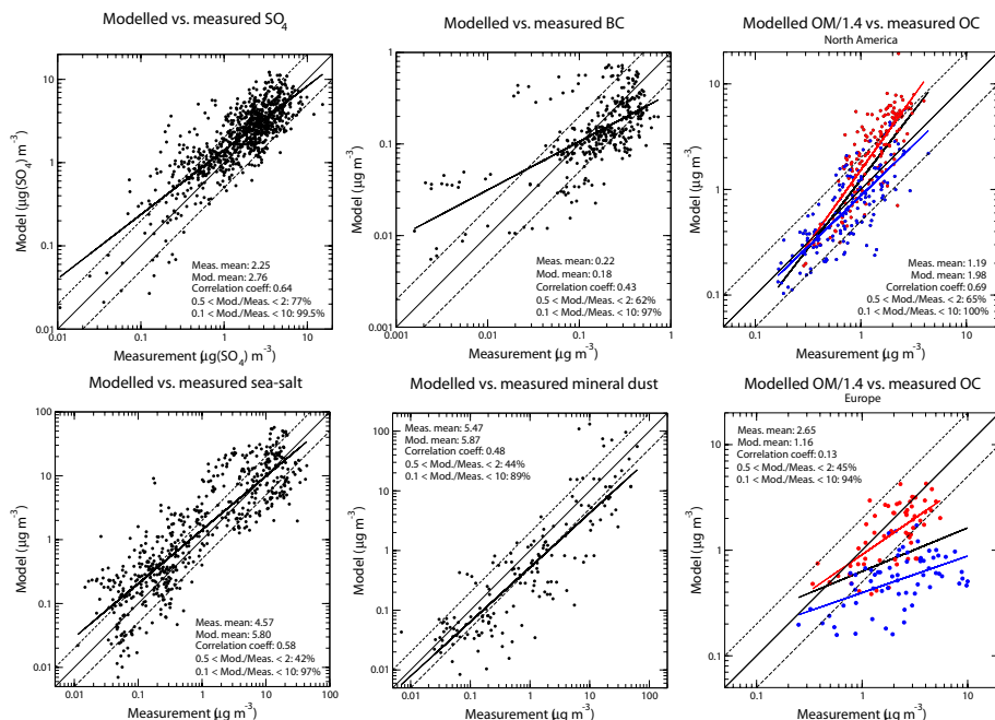
Fig. 4. Modeled versus measured monthly mean ground-level mass concentrations of selected aerosols. The measurements, all from 1996–2002, are made available through the AeroCom project from the AEROCE, AIRMON, EMEP, GAW and IMPROVE measurements networks. The European (EMEP) data are from year 2002, however, and OC data are here given as PM 10 , while the North American OC data are given as PM 2.5 . The European OC measurements have therefore here been scaled by a factor 0.72, to account for the difference between PM 2.5 and PM 10 . The OM data have been split into summer (April–September, red) and winter (October–March, blue). The straight diagonal solid and dashed lines define identical results and a factor 2 difference between the modeled and measured data, respectively. The bold solid lines are regression lines for summer (red), winter (blue) and the full year (black).
