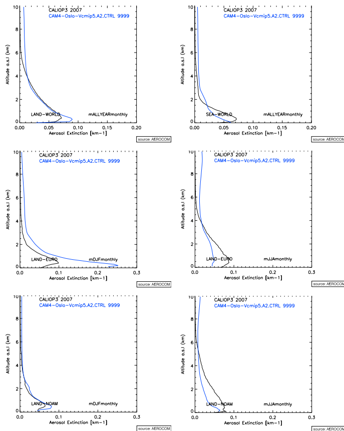
Fig. 10. CAM4-Oslo and CALIOP annually or seasonally averaged extinction coefficient profiles ( \text{km}^{-1} ), continents and oceans globally, and for continental Europe ( 35\text{--}70^\circ\text{N} and 10^\circ\text{W}\text{--}40^\circ\text{E} ) and North America ( 25\text{--}50^\circ\text{N} and 65\text{--}125^\circ\text{W} ) for the winter (DJF) and summer (JJA) seasons. The model data are all-sky estimates at 550 nm, while the CALIOP data are for 532 nm wavelength and for year 2007.
