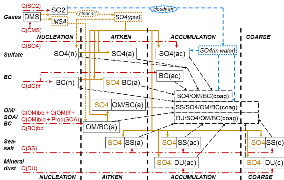
Fig. 1. Schematic for aerosol particle processing in CAM4-Oslo. Primary particles are emitted (dashed-dotted arrows) as accumulation-mode sulphate (SO 4 (ac)), nucleation and accumulation mode black carbon (BC(n), BC(ac)), Aitken mode BC (BC(a)), internally mixed Aitken mode organic matter and BC (OM/BC(a)), Aitken, accumulation, and coarse mode sea-salt (SS(a), SS(ac), SS(c)), accumulation and coarse mode mineral dust (DU(ac), DU(c)). Model calculated gas-phase components are DMS and SO 2 . Gaseous sulphate (SO 4 (gas)) produced in air is assumed transformed to nucleation-mode sulphate (SO 4 (n), dotted arrow) if insufficient particle surface area is available for condensation (solid arrows). Sulphate produced by in cloud water droplets (SO 4 (in water), short-dashed arrow) is partly added to SO 4 (ac) but mainly to a broad internal mixture of accumulation and coarse mode particles (of which there are two types with respect to complexity). Long-dashed arrows represent coagulation which contributes to the latter particle types.
