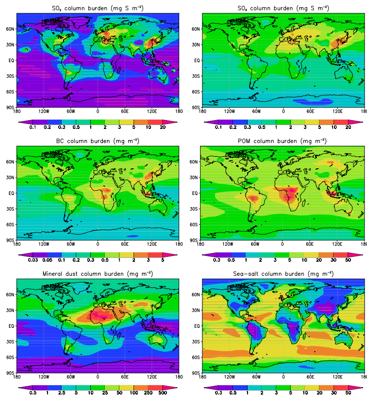
Fig. 2. Annually averaged vertically integrated mass columns of \text{SO}_2 and aerosol constituents in the Ctrl simulation. Globally averaged columns are 0.554 \text{ mg S m}^{-2} for \text{SO}_2 , 1.34 \text{ mg S m}^{-2} for sulphate, 0.466 \text{ mg m}^{-2} for BC, 7.49 \text{ mg m}^{-2} for POM, 23.0 \text{ mg m}^{-2} for mineral dust, and 9.62 \text{ mg m}^{-2} for sea-salt.
