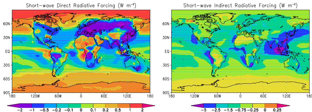
Fig. 11. Modeled annual direct (left, -0.07 \text{ W m}^{-2} ) and indirect (right, -1.20 \text{ W m}^{-2} ) top of the atmosphere short-wave radiative forcing in the control simulations ( Ctrl , years 3–7).
