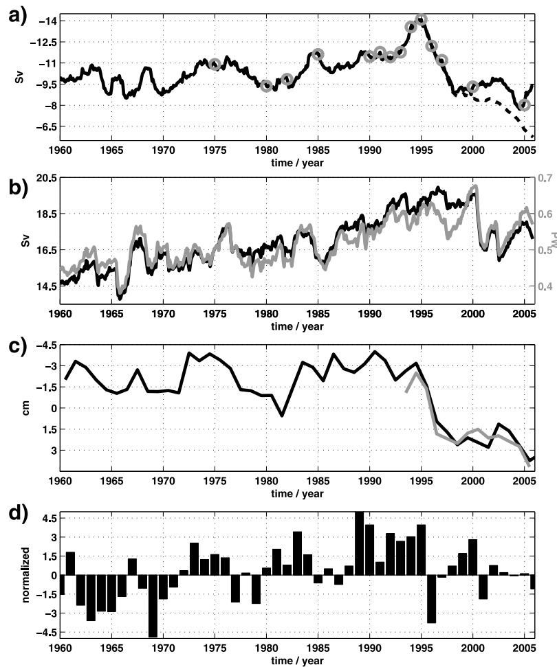
Figure 1. (a) Monthly barotropic streamfunction (Sv; 1 \text{ Sv} = 10^6 \text{ m}^3 \text{ s}^{-1} ) averaged over the North Atlantic SPG region ( 60^\circ\text{W} - 15^\circ\text{W} , 48^\circ\text{N} - 65^\circ\text{N} ) for the control integration (black solid line) and a sensitivity experiment with zero wind stress forcing after 1995 (black dashed line). A one-year running mean filter is applied to the time series. The gray circles indicate the initial conditions in the sensitivity experiments shown in Figure 2. (b) Monthly maximum strength of the AMOC at 41^\circ\text{N} (Sv, black line) and net heat transport across 41^\circ\text{N} (PW, gray line; relative to a temperature of 0^\circ\text{C} ). A one-year running mean filter is applied to the time series. (c) Annual SSH anomalies (cm; with respect to the 1993–1999 mean) for the control integration averaged over the same region as in Figure 1a. The gray line is the corresponding SSH anomalies from the Ssalto/Duacs altimeter data. (d) Observed NAO index defined as difference of normalized winter (December through March, year corresponding to January) SLP between Lisbon, Portugal, and Reykjavik, Iceland. The data were obtained from http://www.cgd.ucar.edu/cas/jhurrel/indices.html .
