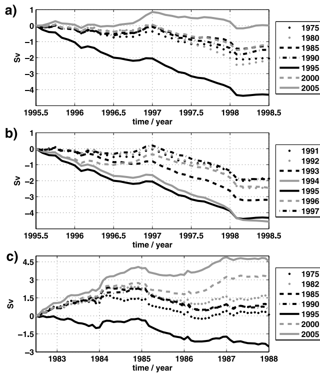
Figure 2. (a) Monthly barotropic streamfunction anomalies (Sv; with respect to the initial value) averaged over the North Atlantic SPG region ( 60^{\circ}\text{W} – 15^{\circ}\text{W} , 48^{\circ}\text{N} – 65^{\circ}\text{N} ) for the sensitivity experiments in which the post 1995 atmospheric forcing is applied to ocean initial conditions every five years between and including 1975 and 2005. Line style according to legend. A one-year running mean filter is applied to the time series. The 1995 ocean initial condition is the control integration. (b) Same as Figure 2a but for ocean initial conditions every year between and including 1991 and 1997. (c) Same as Figure 2a but for the sensitivity experiments in which the post 1982 atmospheric forcing is applied. Note that the 1982 ocean initial condition is the control integration.
