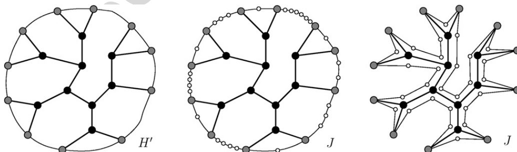
Fig. 5. The transformation of the proof of Lemma 8.
