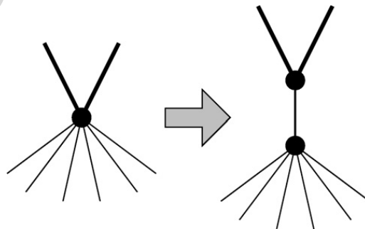
Fig. 4. Step 2 of the algorithm in Lemma 7.
