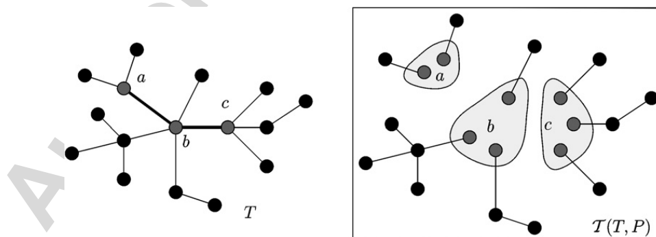
Fig. 1. An example of the definition of the graph collection \mathcal{T}(T, P) for some tree T and some path P = (a, b, c) in it.
