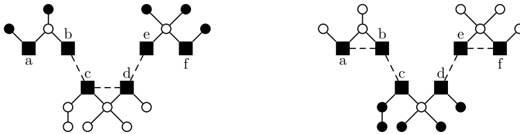
Fig. 4 The two subproblems corresponding to the instance of Fig. 3. For visualization reasons, we drew only the edges of ST , plus the edges in F \cup E_2 and F \cup E_1 (dashed edges on the left and right, respectively)
