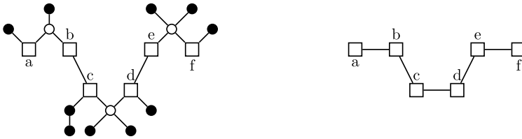
Fig. 3 On the left, a Steiner tree ST of a graph G . (The other edges of G are not depicted for visualization reasons.) Black nodes denote terminals. Squared nodes define a perfectly-balanced separator S = \{a, b, c, d, e, f\} . The nodes above and below S define the node sets V_1 and V_2 , respectively. In particular, T_1 and T_2 are given by the top and bottom black nodes, respectively. Observe that ST_1 = ST[V_1 \cup S] is a forest. On the right, the corresponding tree ST' . In particular, F = \{bc, de\} , E_1 = \{ab, ef\} , and E_2 = \{cd\}
