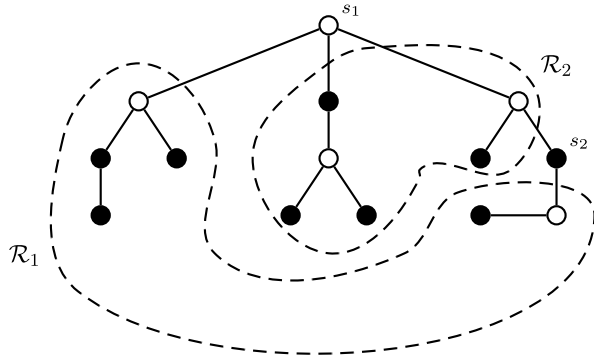
Fig. 2 A perfectly-balanced separator S = \{s_1, s_2\} , of size 2 \leq \log 9 + 1 , and the corresponding forests \mathcal{R}_1 and \mathcal{R}_2 , each one containing 4 \leq 9/2 terminals
