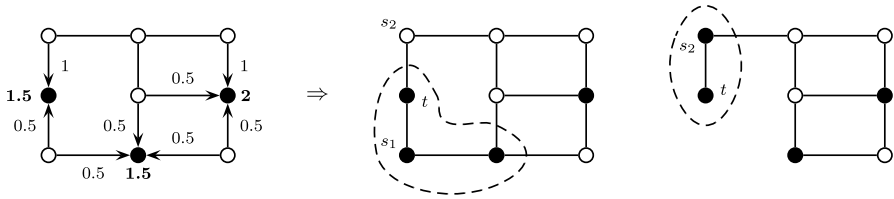
Fig. 5 Assignment of load to terminals (black nodes) on the left, and multiple branching on the minimum load terminal t : in the first subproblem s_1 is added to the terminals (middle); in the second s_1 is deleted and s_2 is added to the terminals (right). Dashed curves indicate components of terminals which will be contracted in the following step.
