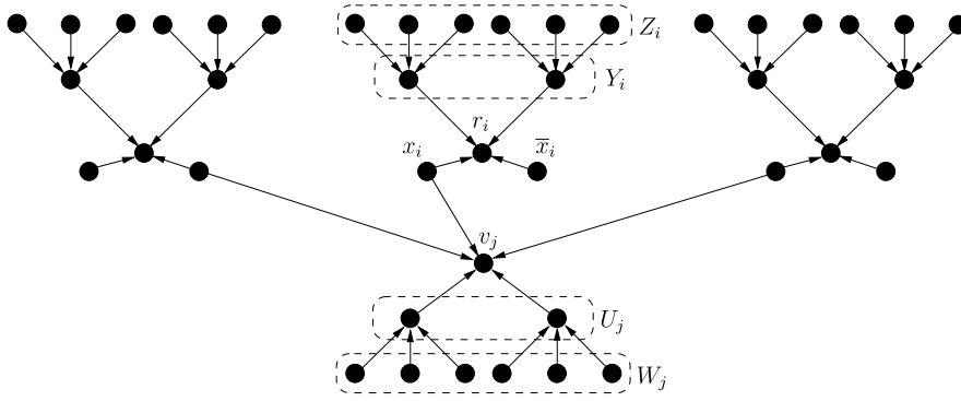
Fig. 1. Construction of G for k=3 .
