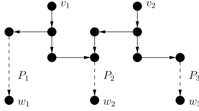
Fig. 2. Construction of G for U = \{u_1, u_2, u_3\} and X_1 = \{u_1, u_2\} , X_2 = \{u_2, u_3\} .
