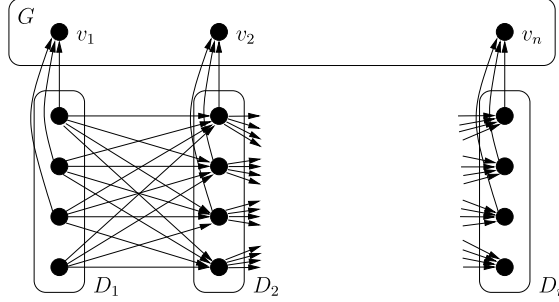
Fig. 3. Construction of G' for k=4 .
