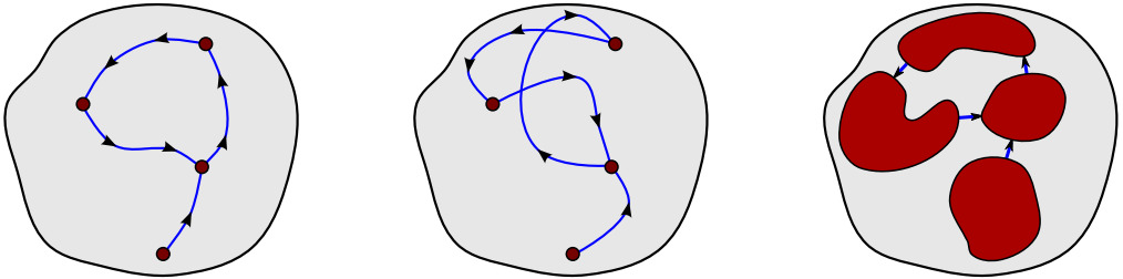
Fig. 2. Expansion, immersion, and a minor model of the same 4-vertex digraph H in a larger digraph G .
