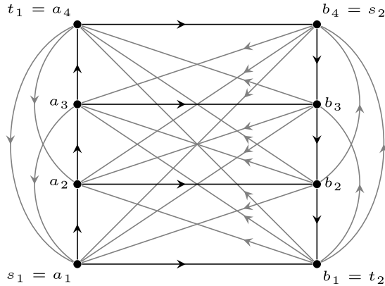
Fig. 5. Tournament T_4 .
