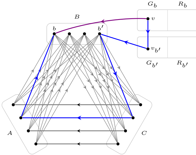
Fig. 4. Rerouting strategy for a path accessing vertex b from G_b . The original path is depicted in violet, while the rerouted path is depicted in blue. (For interpretation of the colors in the figure(s), the reader is referred to the web version of this article.)
