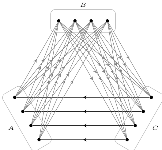
Fig. 3. A 4-triple.
