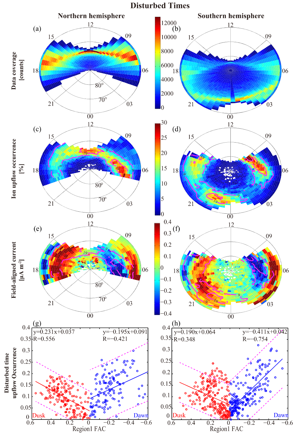
Figure 3. Same format as Figure 2 but for magnetic disturbed times.
