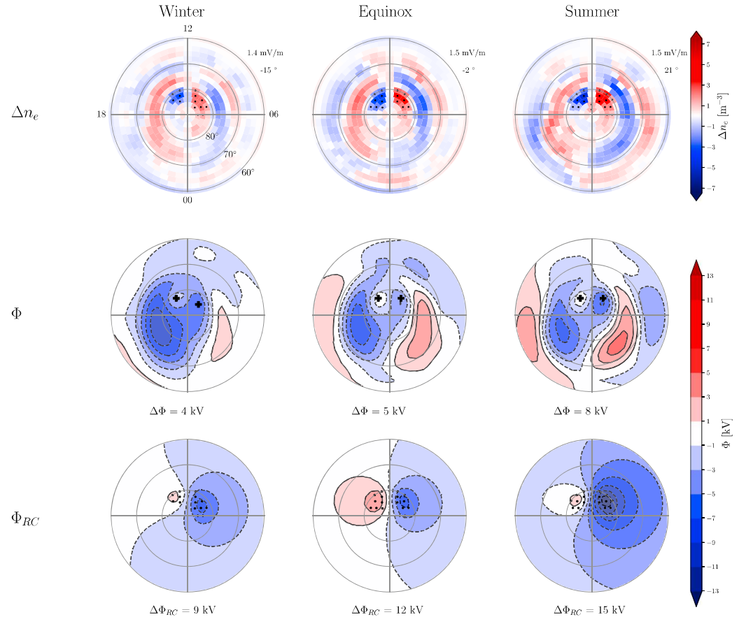
Figure 3. Inferred reverse convection potential \Phi_{RC} from the Northern Hemisphere during northward interplanetary magnetic field (IMF) for three different dipole tilt intervals based on Super Dual Auroral Radar Network line-of-sight measurements: (left column) winter (dipole tilt less than -10^\circ ), (middle column) equinox (dipole tilt within \pm 10^\circ ), and (right column) summer (dipole tilt > 10^\circ ). The upper row shows the inferred \Delta n_e from the Spherical Elementary Convection Systems analysis, with reverse convection grid cells indicated with black dots. The middle row shows the electric potential \Phi . The bottom row shows the electric potential resulting from the selected reverse convection grid cells only. This potential is what we relate to the lobe reconnection rate and is printed below each panel.
