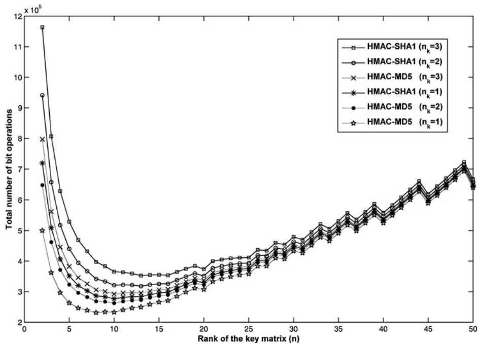
Figure 6. Required number of operations for encrypting a plaintext of L = 400 letters for different rank values when the modulus p is fixed ( p=29 ).
