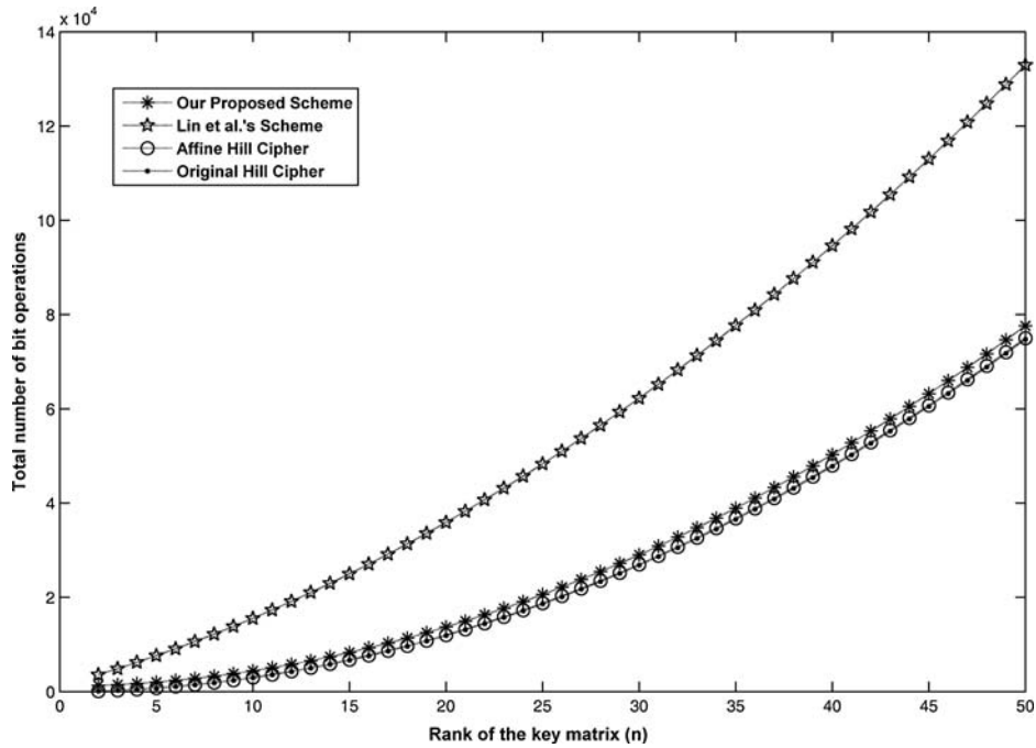
Figure 5. Required number of operations for encrypting each block of data for different rank values when the modulus p is fixed ( p=29 ).
