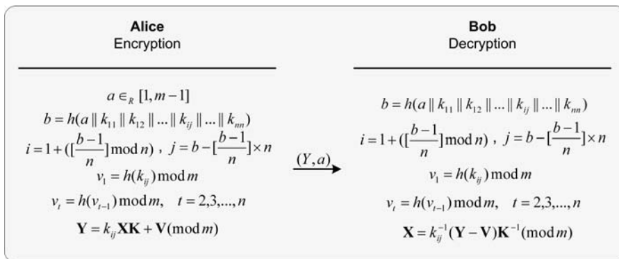
Figure 1. The corrected Lin et al. 's scheme [9].
