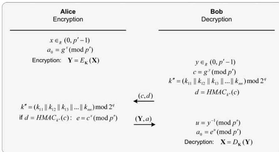
Figure 3. A two-pass protocol for the proposed cryptosystem (Protocol 'A').
