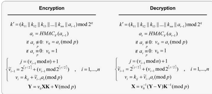
Figure 2. Encryption core of the proposed cryptosystem.
