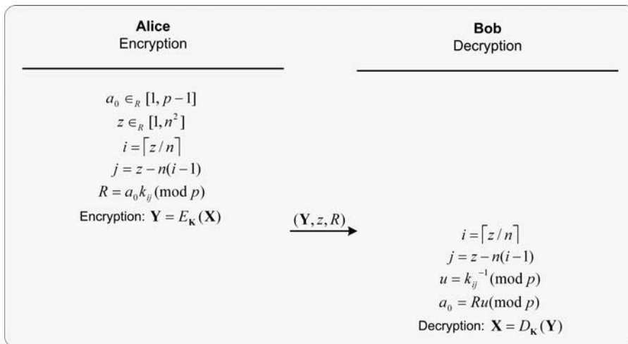
Figure 4. A one-pass protocol for the proposed cryptosystem (Protocol 'B').
